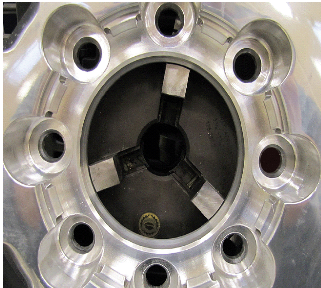
Hunter TruckChuck® Correctly Attached (Close Up)
