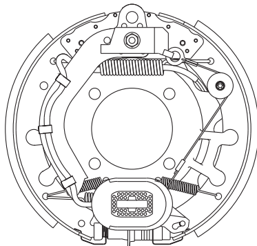
New Style Brake Cast Backing Plate
