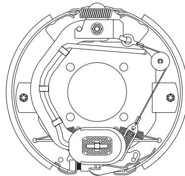
Old Style Brake Stamped Backing Plate
