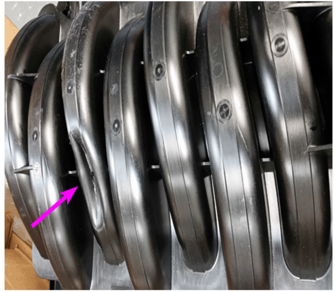
View of Intake from GEN 5 V8 that Experience Lifter Collapse and/or Broken Valve Spring
