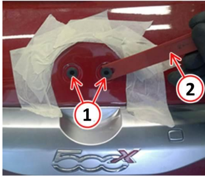
Fig. 3 Remove And Discard Emblem Fasteners
