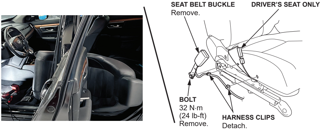
POWER SEAT WITHOUT VENTILATED SEAT
