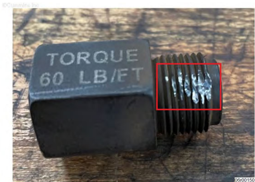
Figure 6, Seal Installer Tool Threads Not Acceptable for Use.
