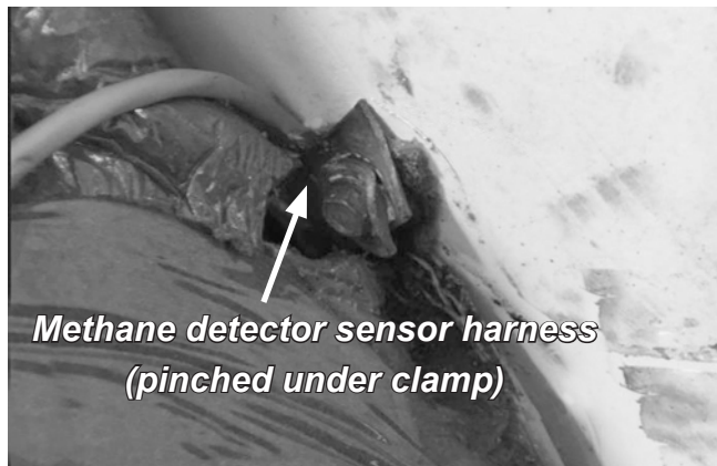
Figure 5, Methane detector sensor harness (damaged)
