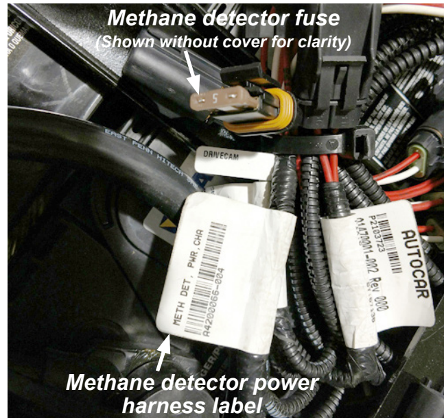
Figure 2, Methane detector fuse
