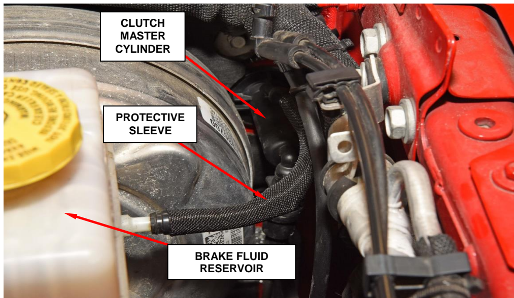
Figure 2 – Hose Sleeve Installed
