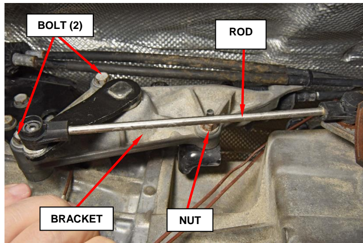
Figure 11 – Rod Bracket
