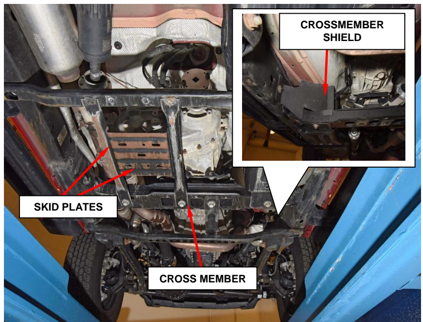
Figure 6 – Skid Plates
