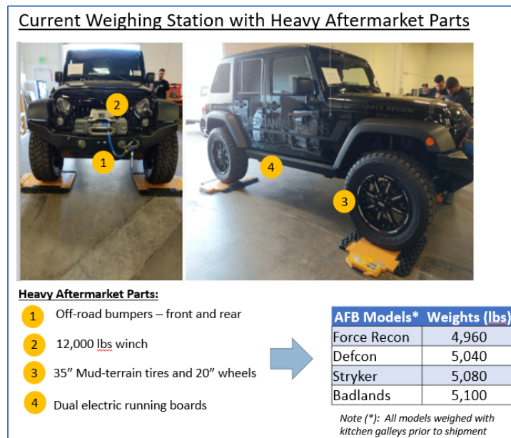
Figure 1: Vehicle Weighing Station
