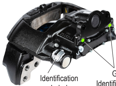
Bendix® ADB22X™ Air Disc Brake
