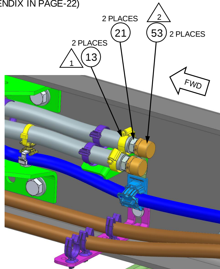
AIR & SPRING SUSPENSION, REAR CHARGE PORT
