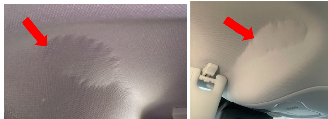
Fig. 1 Headliner Delamination (Bubbling) Examples
