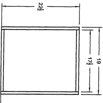
Shelf A - \frac{1}{8} " Wood Panel Top View \frac{3}{4} x \frac{3}{4} Lumber Cleats Staple This Side 1 - Required
