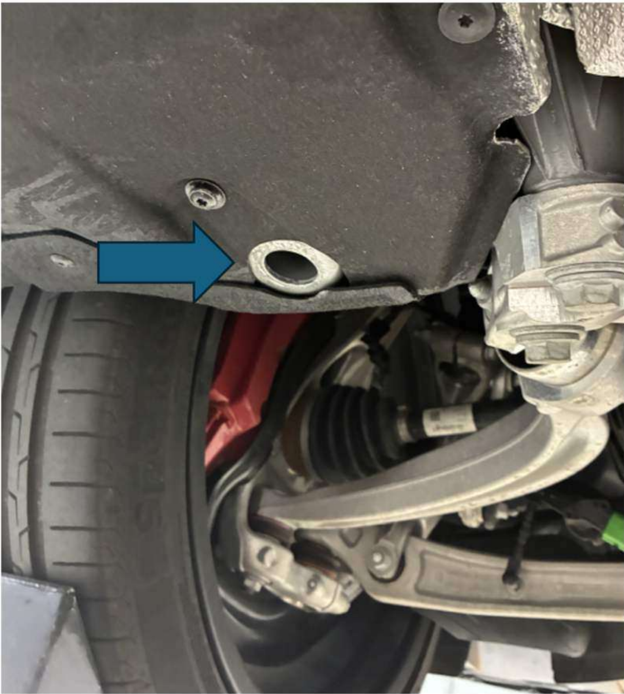
Figure 1. Plug (part number 4M0.899.183.A) missing in area of pick-up point
