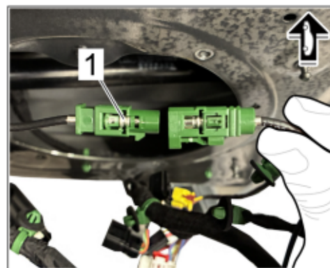
Example illustration of plug contact on mirror side
