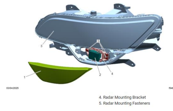
Fig. 4, Front Radar Removal
